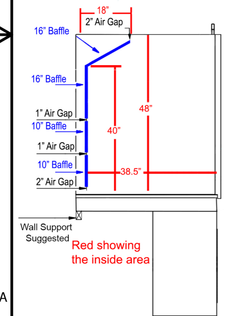
LEFT SIDE VIEW SASH OPEN
