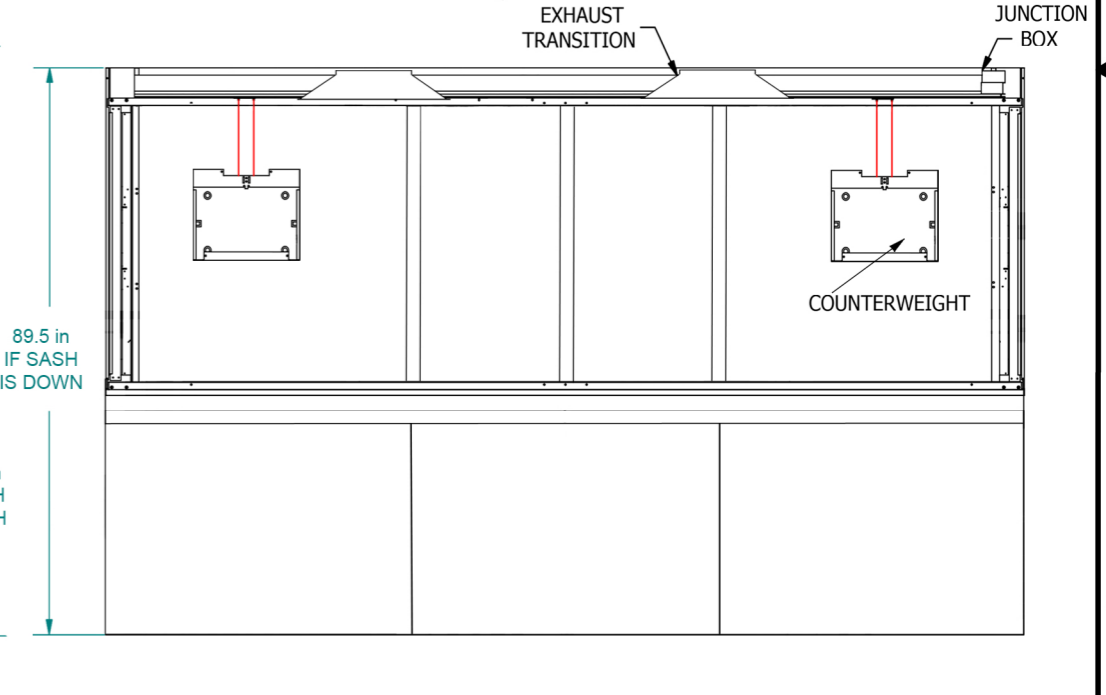
BACK VIEW SASH CLOSED
