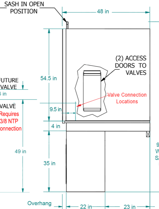
RIGHT SIDE VIEW SASH OPEN
