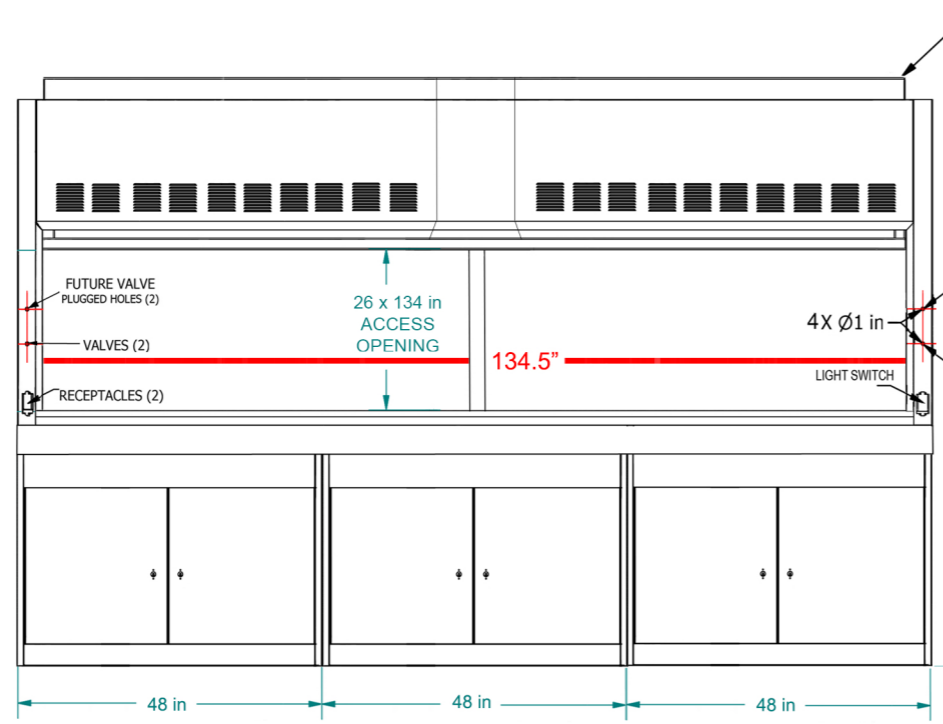
FRONT VIEW SASH OPEN
