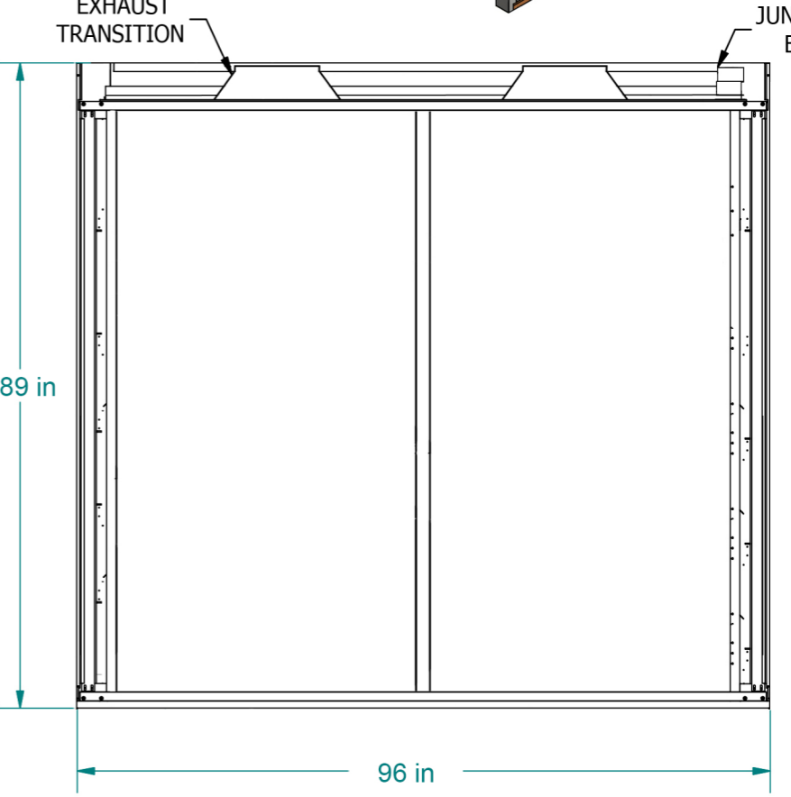
BACK VIEW SASH CLOSED
