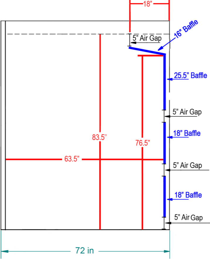
RIGHT SIDE VIEW SASH OPEN
